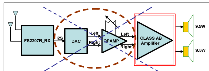
Typical Wireless Class AB Amp Solution
